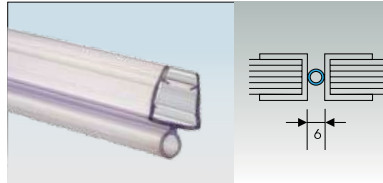
OPS-5 8mm STD ₹ 315 OPS-5 10mm STD ₹ 315 Soft Nose Seal
