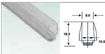
OPS-SL-BR-11 10mm STD ₹ 819 OPS-SL-BR-11 12mm STD ₹ 971 Brush Seal (Central)
