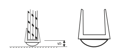
Glass to Floor / Wall For 8/10/12mm Size-2200mm Finish-Transparent EGP 510 - 08 ₹350.00 EGP 510 - 10 ₹350.00 EGP 510 - 12 ₹350.00
